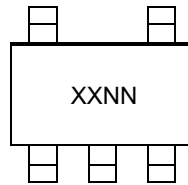
5-Lead SC70 (MCP6L01)
