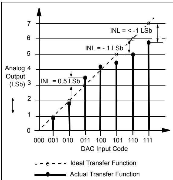
FIGURE C-4: INL Accuracy.
