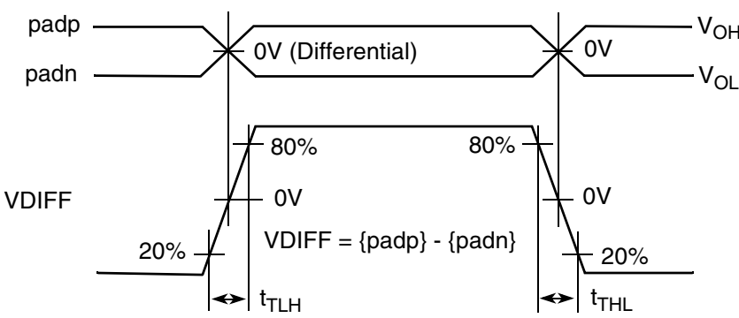
Figure 7. Differential MLB Driver Transition Time Waveform
