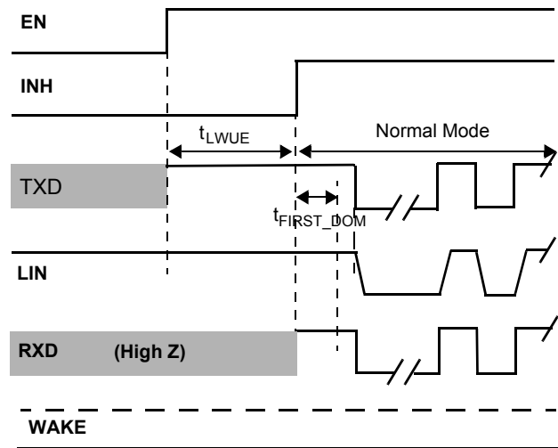
Figure 14. EN Pin Wake-up with TXD High
