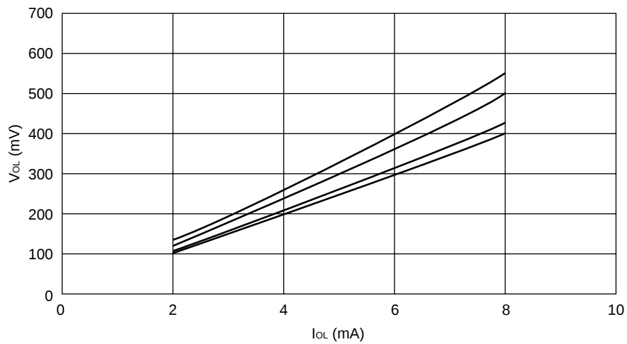
V_{OL} - I_{OL} Other than P20 to P27
