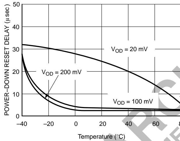
Figure 6. Power-Down Reset Delay vs. Temperature (MAX81xR/S/T/F)
