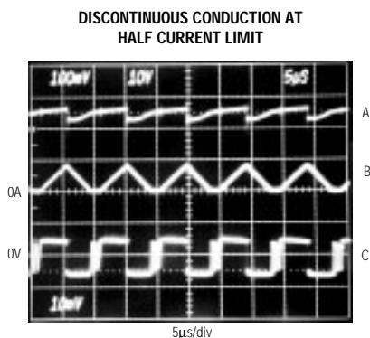
CIRCUIT OF FIGURE 2, V_+ = 5V , V_{OUT} = -5V , I_{LOAD} = 80mA A: OUTPUT RIPPLE, 100mV/div B: INDUCTOR CURRENT, 500mA/div C: LX WAVEFORM, 10V/div
