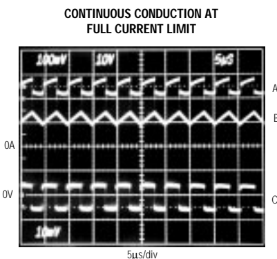
CIRCUIT OF FIGURE 2, V_+ = 5V , V_{OUT} = -5V , I_{LOAD} = 240mA A: OUTPUT RIPPLE, 100mV/div B: INDUCTOR CURRENT, 500mA/div C: LX WAVEFORM, 10V/div
