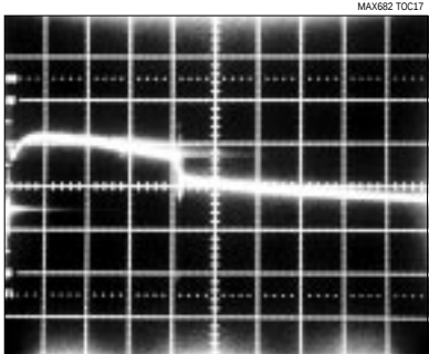
OUTPUT WAVEFORM (SKIP = LOW)
