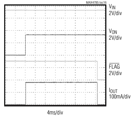
FLAG-BLANKING RESPONSE
