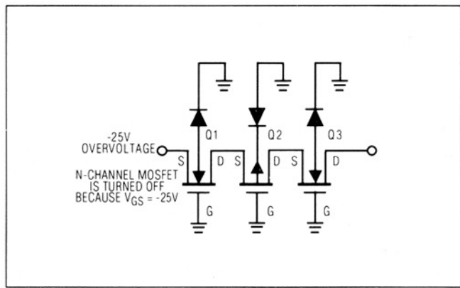
Figure 9. +25\text{V} Overvoltage with Multiplexer Power OFF
