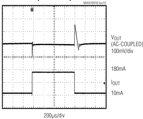
LOAD-TRANSIENT RESPONSE (5V OUTPUT)
