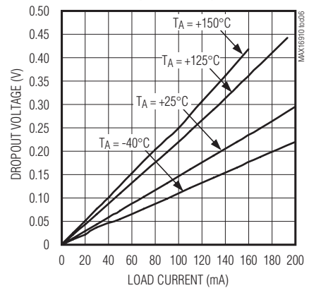
DROPOUT VOLTAGE vs. LOAD CURRENT (5V OUTPUT)
