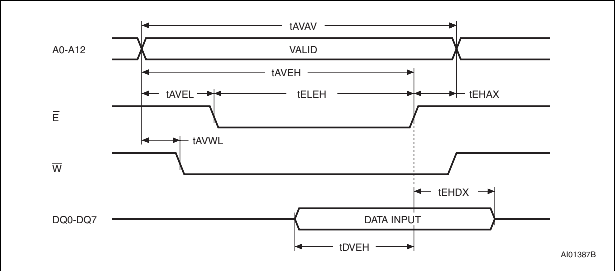
Figure 6. Chip enable controlled, WRITE mode AC waveforms
