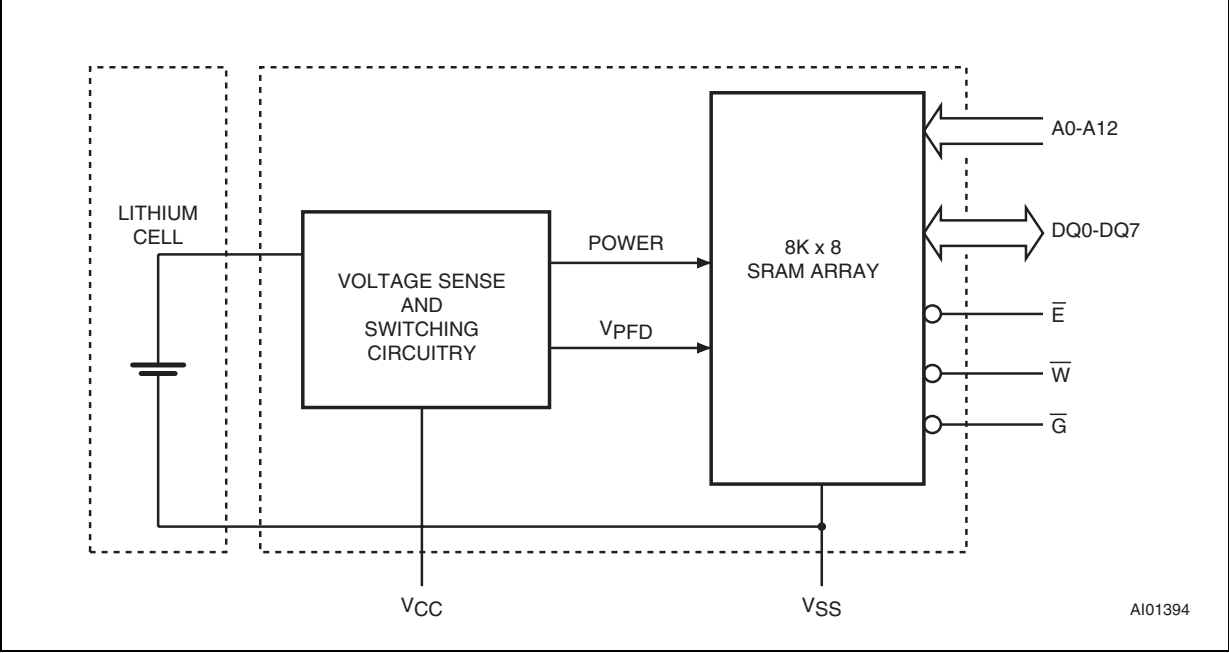
Figure 3. Block diagram
