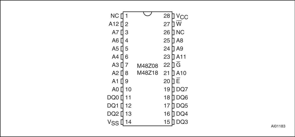
Figure 2. DIP connections
