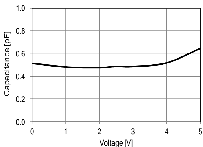
Voltage—Capacitance Characteristic
