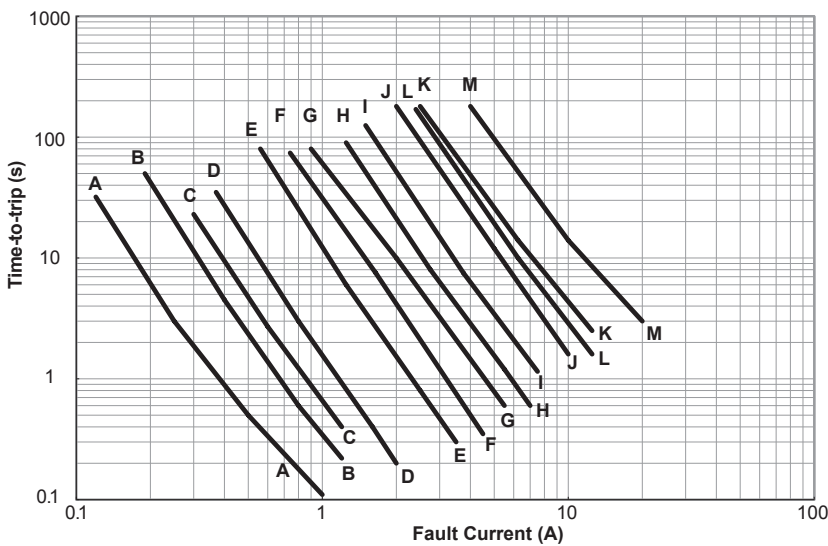
Figure L8 — Typical Time-to-Trip Curves at 20°C
