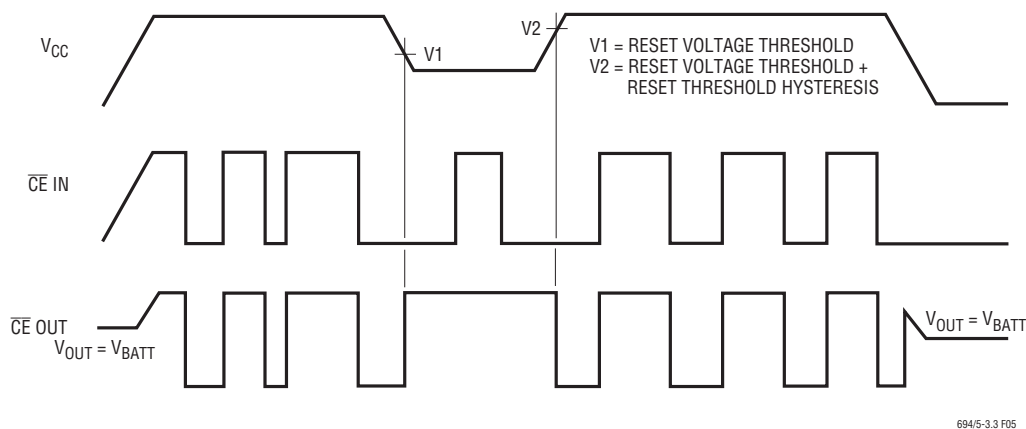
Figure 5. Timing Diagram for \text{C}\overline{\text{E}} \text{ IN} and \text{C}\overline{\text{E}} \text{ OUT}
