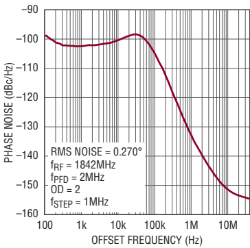
LTC6946-2 Mixer Application Phase Noise
