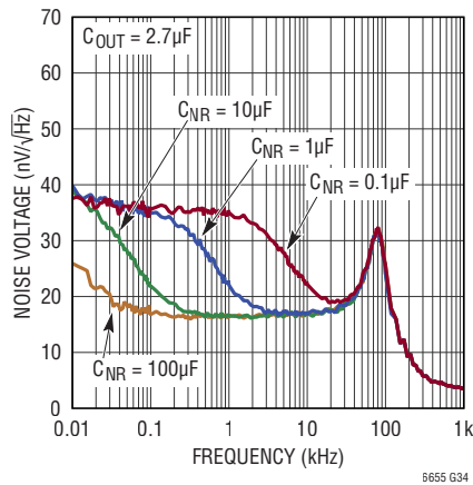
LTC6655LN-2.5 Output Voltage Noise Spectrum
