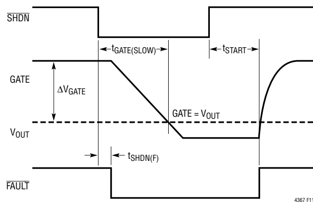
Figure 11. Shutdown Timing
