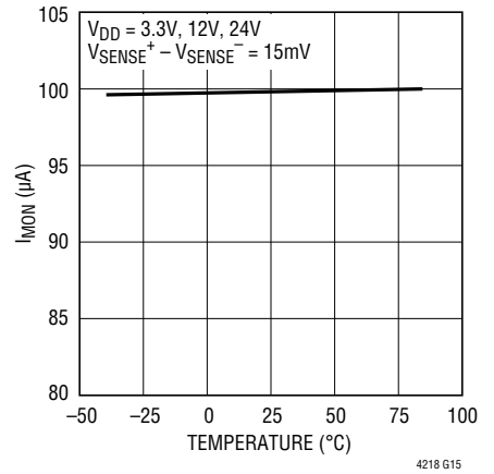
I_{\text{MON}} vs Temperature and V_{DD}
