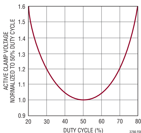
Figure 8. V_{CL} Voltage vs Duty Cycle
