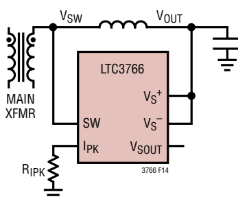
Figure 14b. Setting R_{IPK} with No Differential Amplifier
