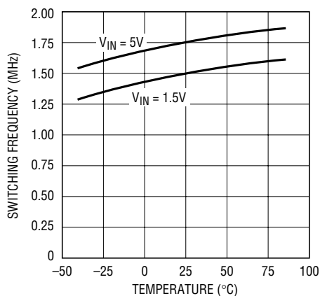
Boost Converter Oscillator Frequency vs Temperature
