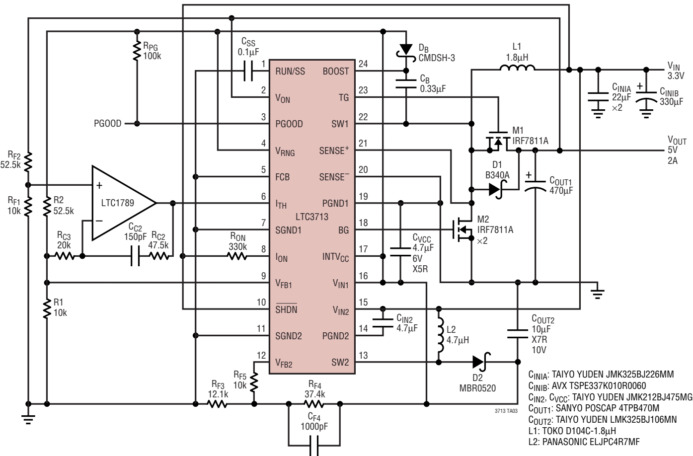
3.3V to 5V Synchronous Boost Converter
