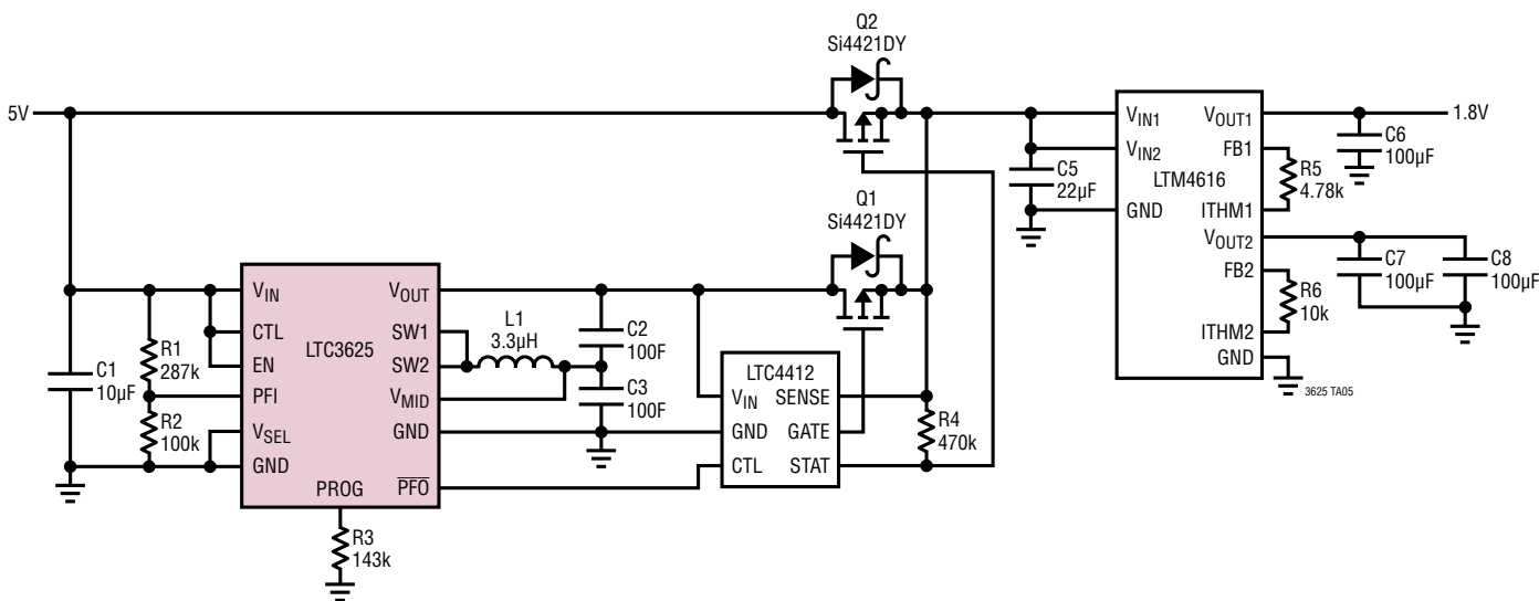
5V Power Ride-Through
