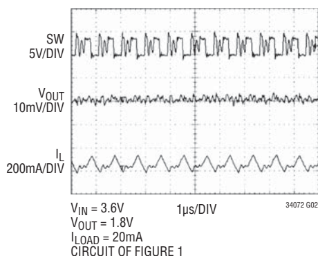
Pulse-Skipping Mode
