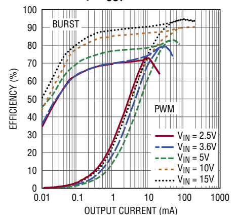
Efficiency, V_{OUT} = 15\text{V}
