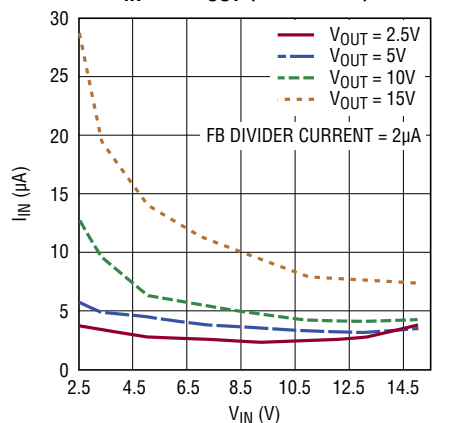
No Load Input Current vs V_{IN} and V_{OUT} (PWM = 0V)
