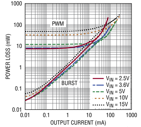
Power Loss, V_{OUT} = 5\text{V}
