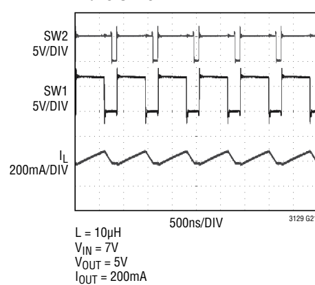
Fixed Frequency PWM Waveforms
