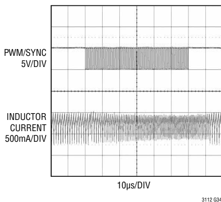
1500kHz SYNC Signal Capture and Release
