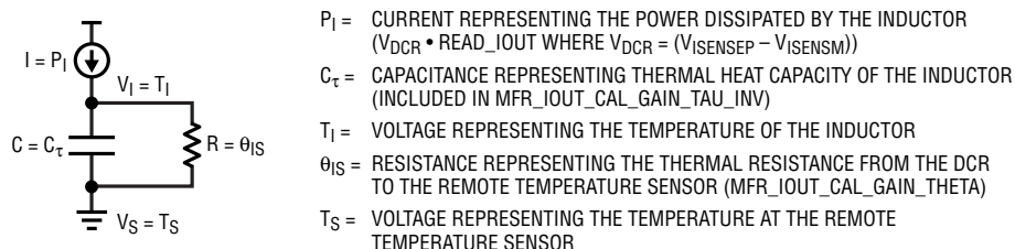
Figure 21. Electronic Analogy for Inductor Temperature Model
