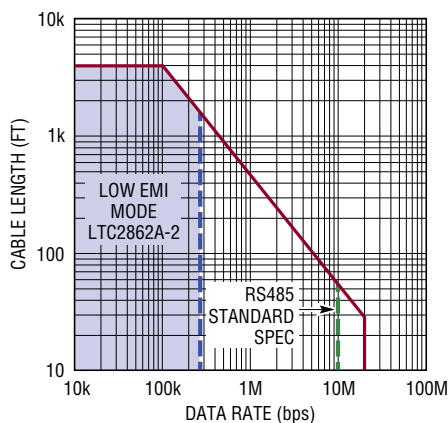
Figure 10. Cable Length vs Data Rate (RS485/RS422 Standard Shown in Vertical Dashed Line)
