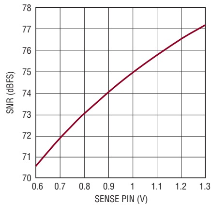
LTC2191: SNR vs SENSE, f_{IN} = 5\text{MHz} , -1dBFS
