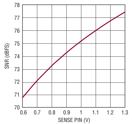
LTC2190: SNR vs SENSE, f_{IN} = 5\text{MHz} , -1\text{dBFS}
