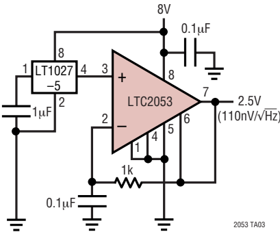
Precision \div 2 (Low Noise 2.5V Reference)
