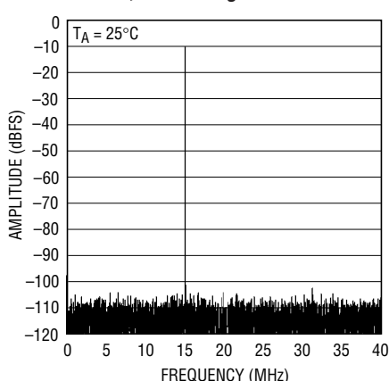
8192 Point FFT, Input Frequency = 15.068MHz, -10dB, 3.2V Range
