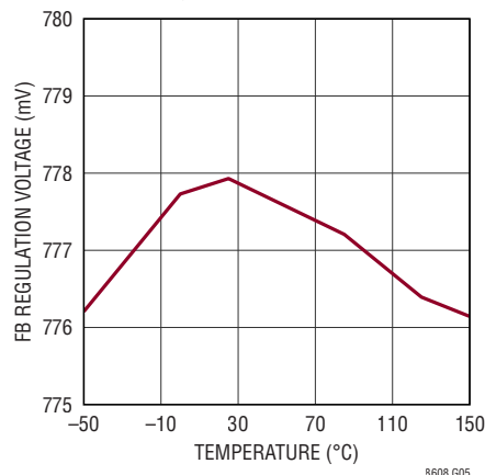
FB Voltage
