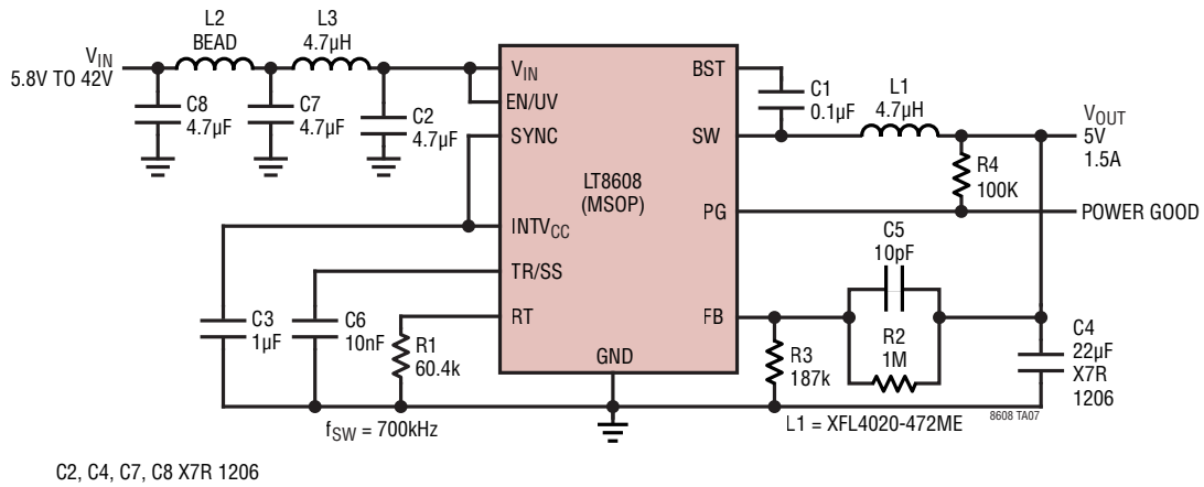
Ultralow EMI 5V 1.5A Step-Down Converter
