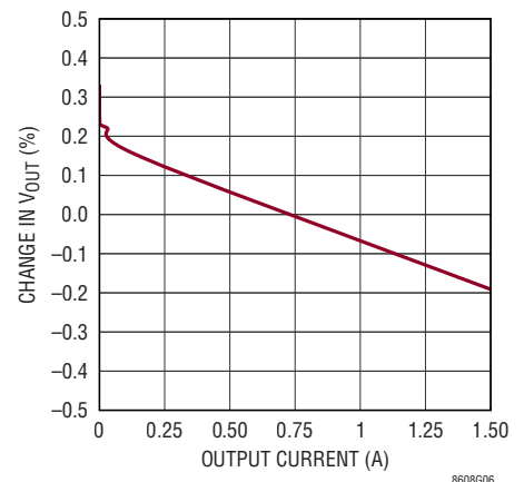
Load Regulation
