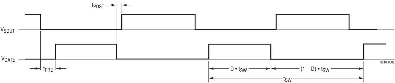
Nonoverlapping GATE/SOUT
