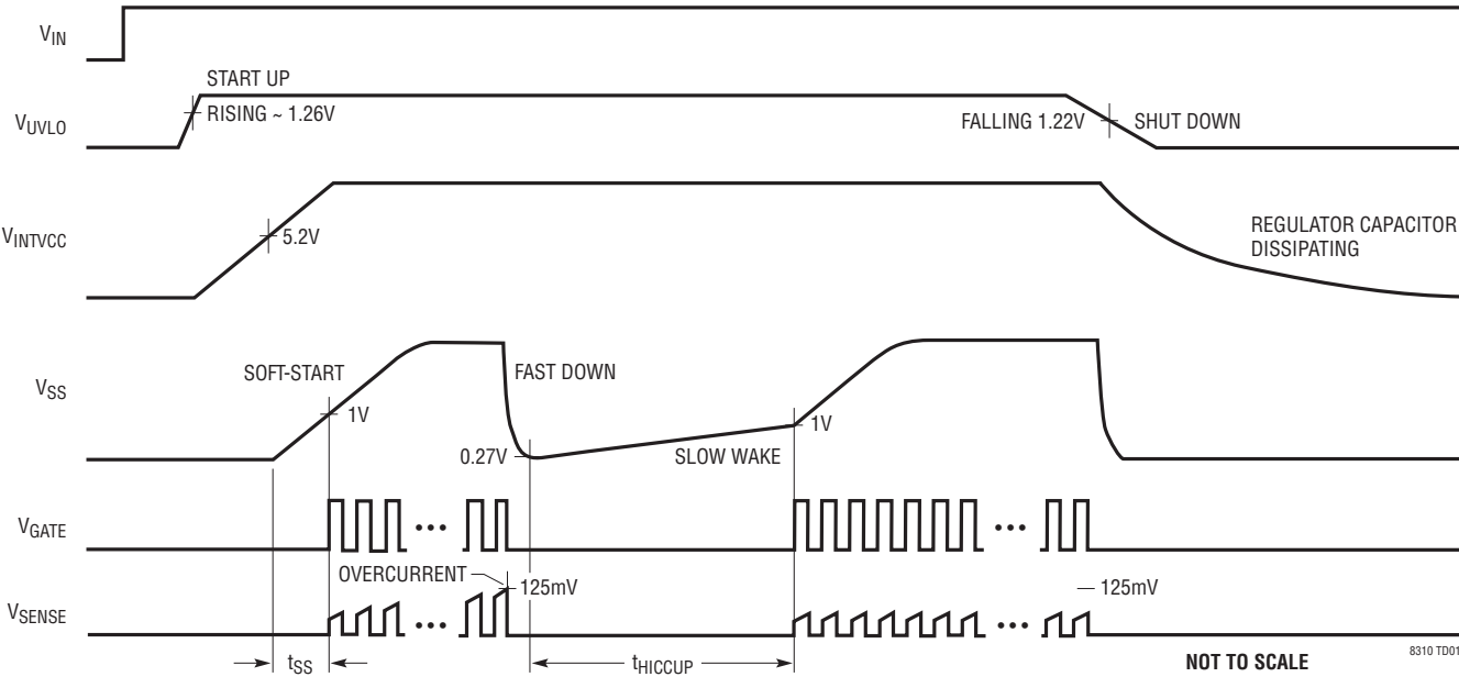
Start-Up/Soft-Start/Fault/Shutdown/Restart
