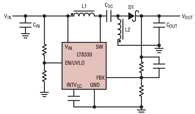
Figure 5. LT8330 Configured in a SEPIC Topology
