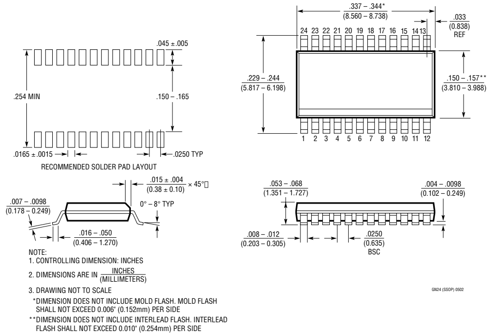
GN Package 24-Lead Plastic SSOP (Narrow .150 Inch) (Reference LTC DWG # 05-08-1641)
