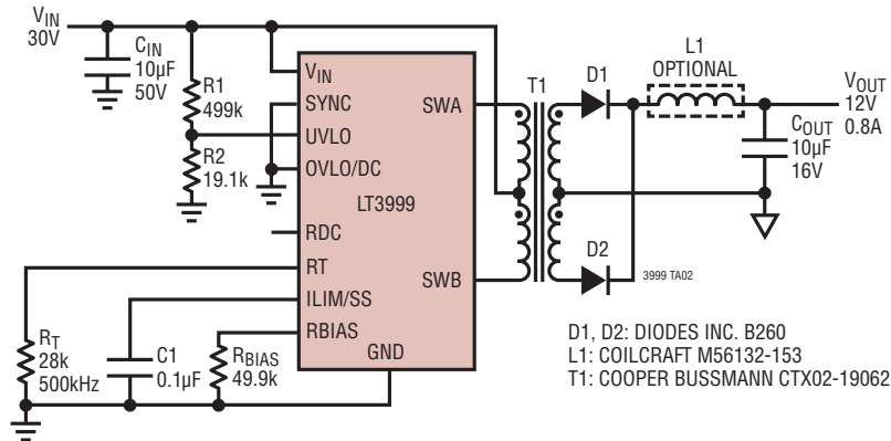
30V to 12V, 10W Push-Pull DC Transformer
