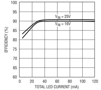
Efficiency vs Total LED Current
