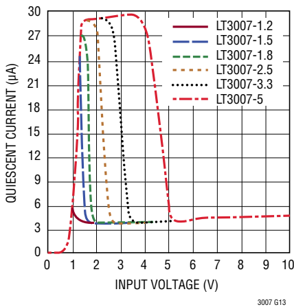
Quiescent Current
