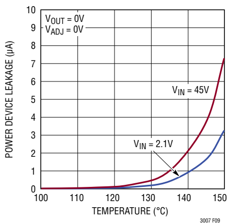
Figure 9. Power Device Leakage, \overline{\text{SHDN}} = 0\text{V}
