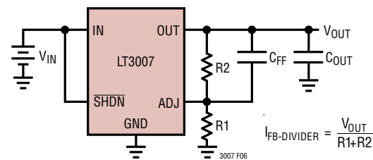
Figure 6. Feedforward Capacitor
