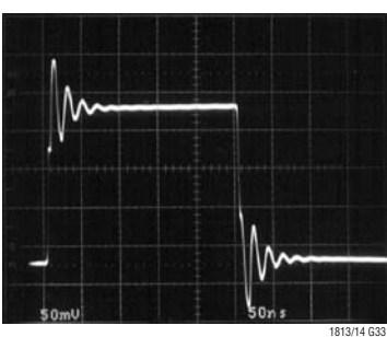
Small-Signal Transient ( A_V = 1 , C_L = 100\text{pF} )
