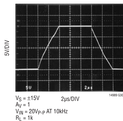
±15V Large-Signal Response
