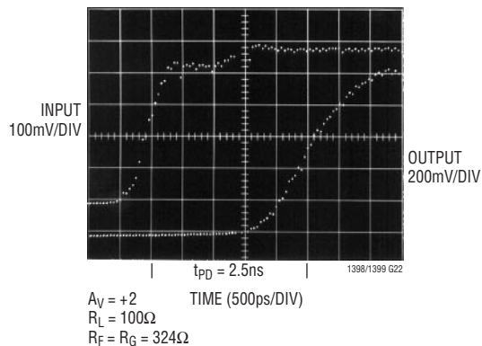
Propagation Delay
