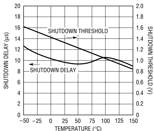
Shutdown Delay and Threshold vs Temperature
