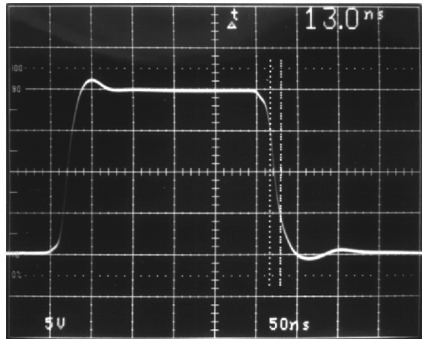
Figure 5a. Large-Signal Response, A_V = 1
