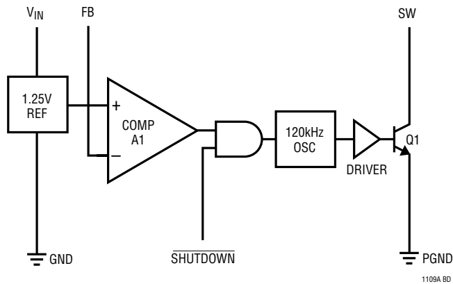
LT1109A (Adjustable)
