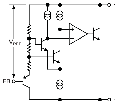
LM4041 Adjustable
