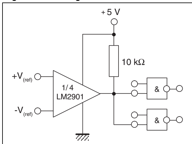
Figure 10. Driving TTL
