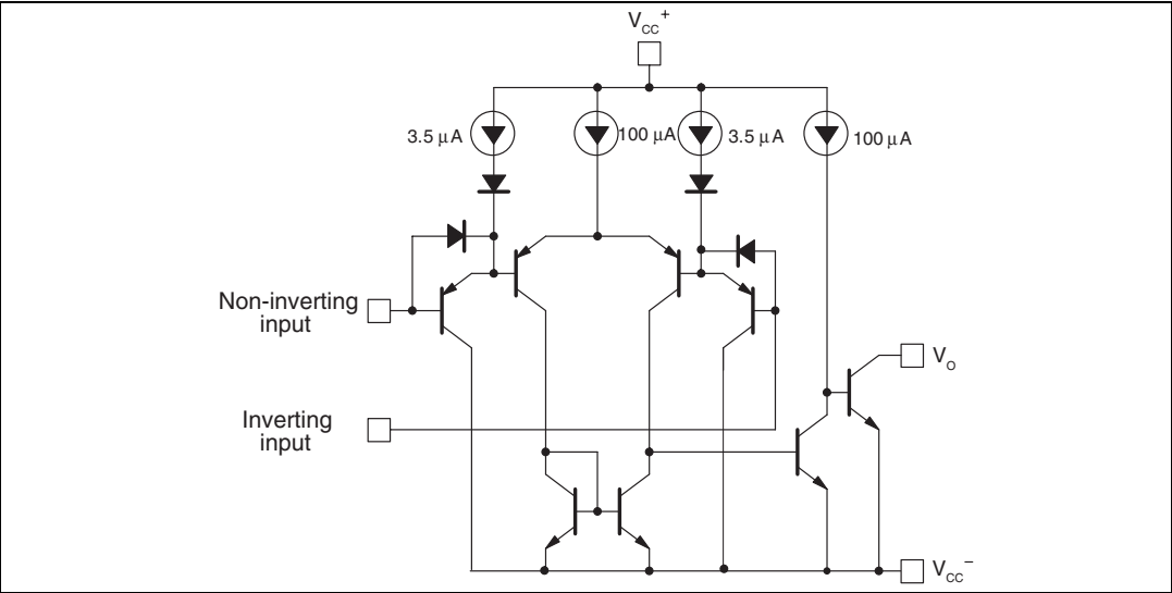
Figure 2. Schematic diagram
