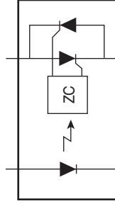
Zero-Cross Turn-On
