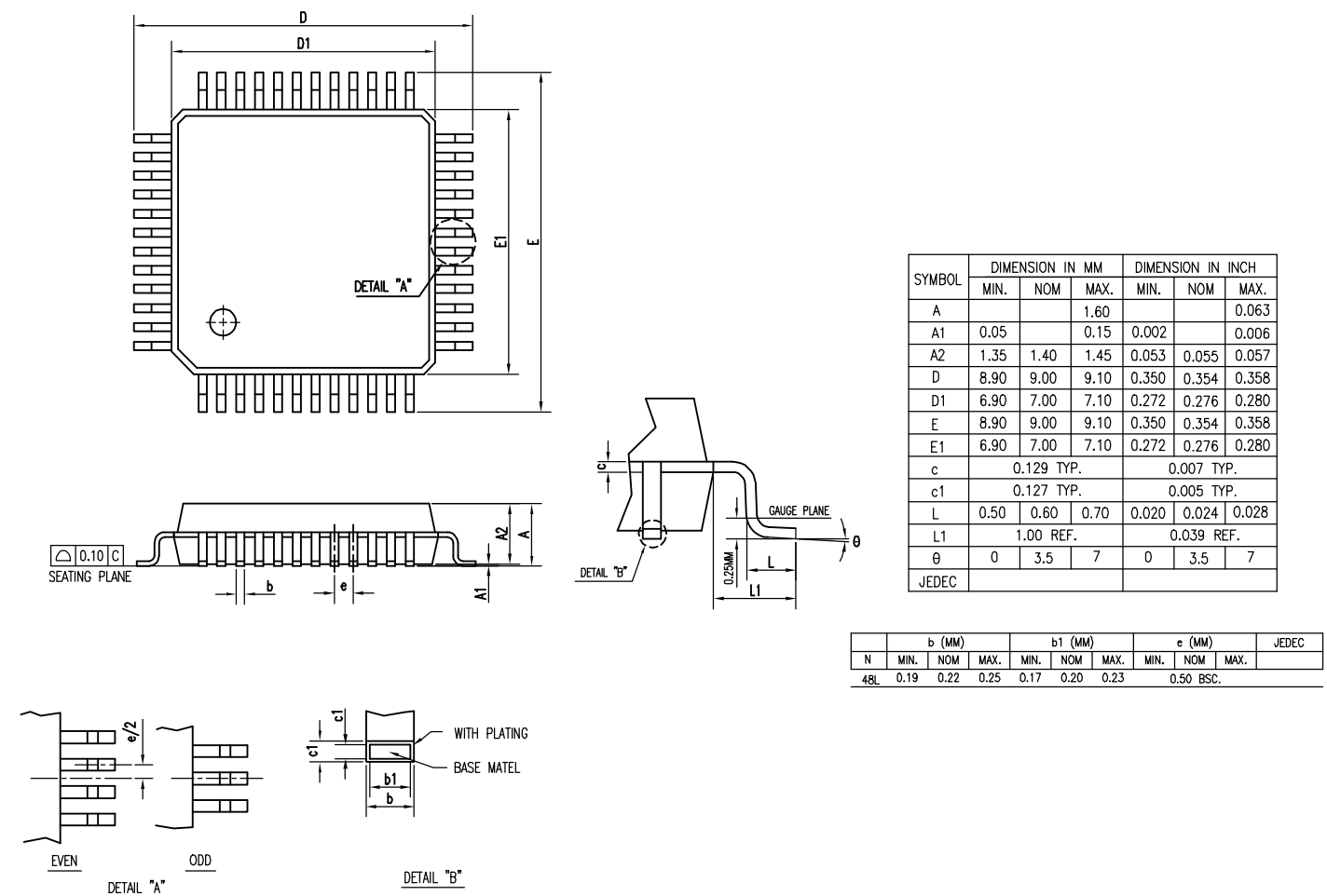
48-Pin (7mm x 7mm) LQFP
