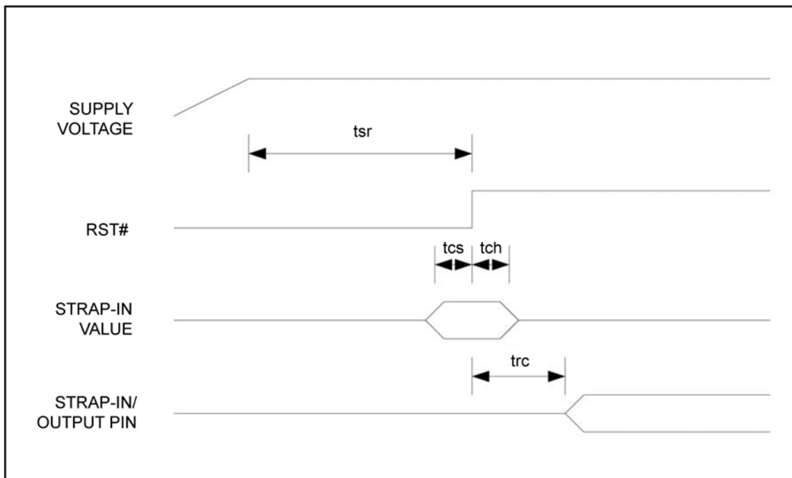
Figure 14. Reset Timing
