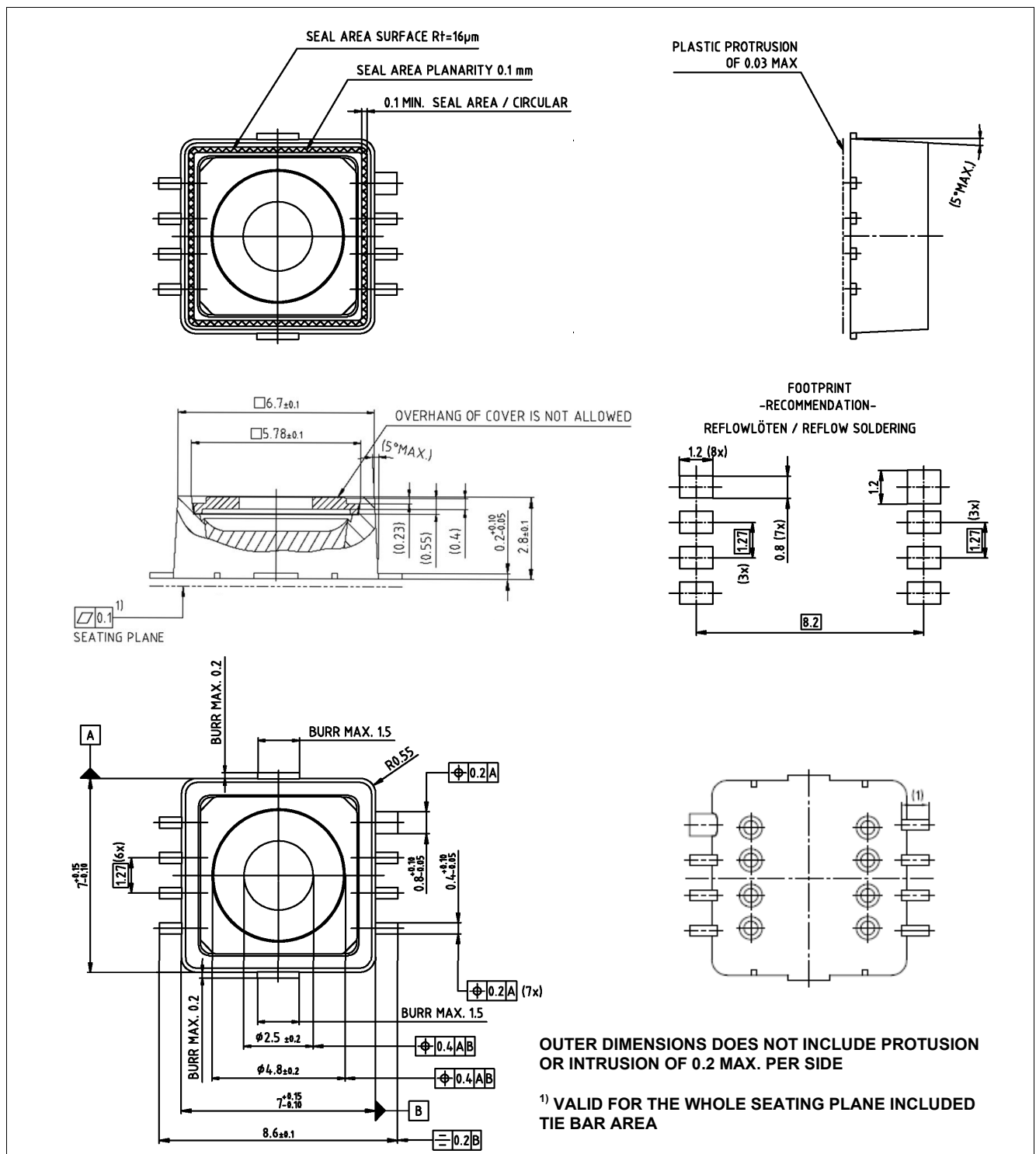
Figure 26 Package outline
