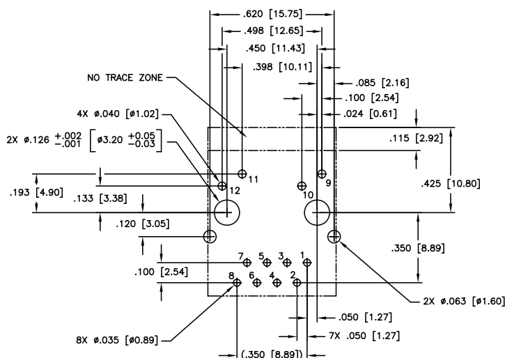
View from PCB component side
