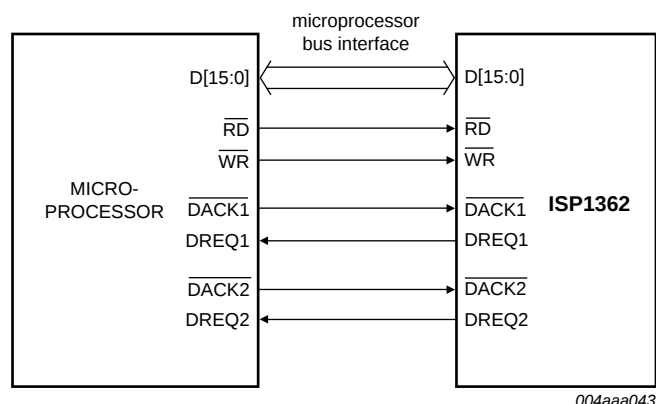
Fig 9. DMA interface between a microprocessor and the ISP1362
