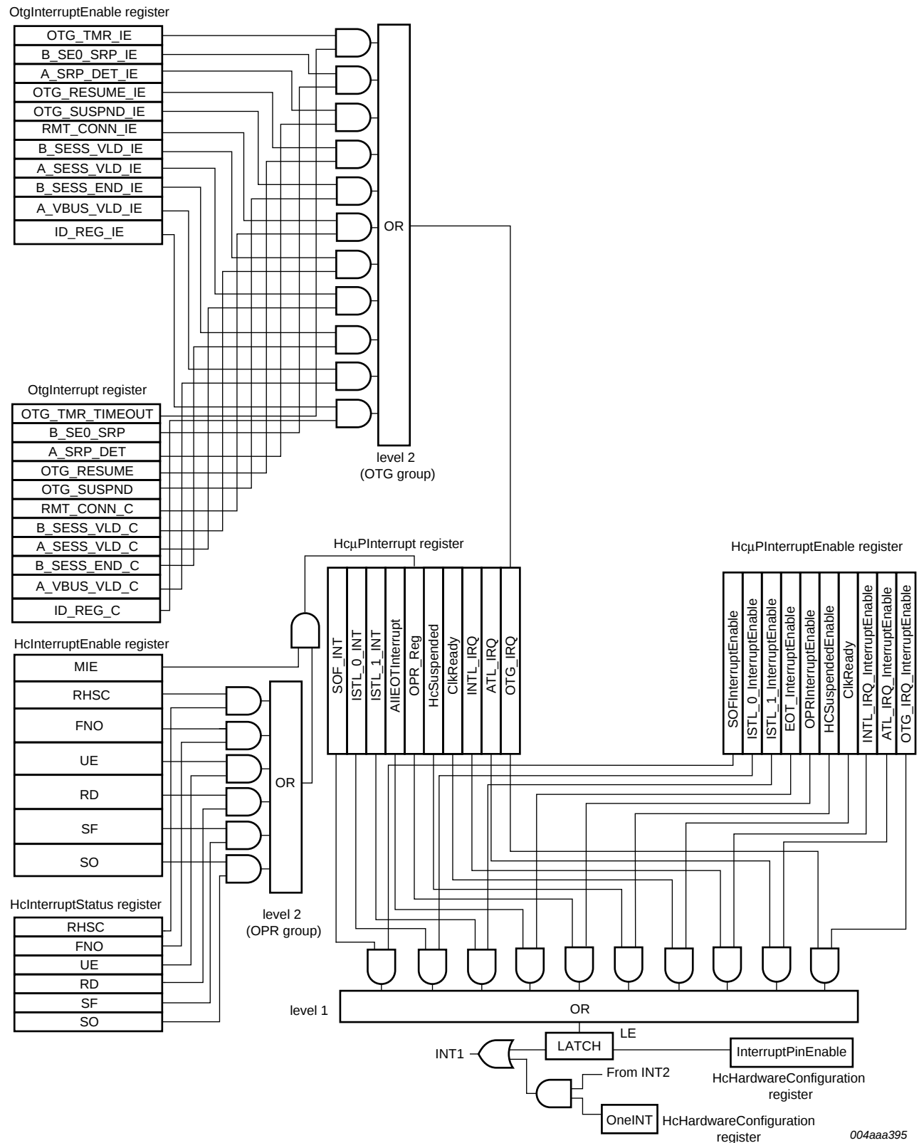
Fig 14. HC and OTG interrupt logic
