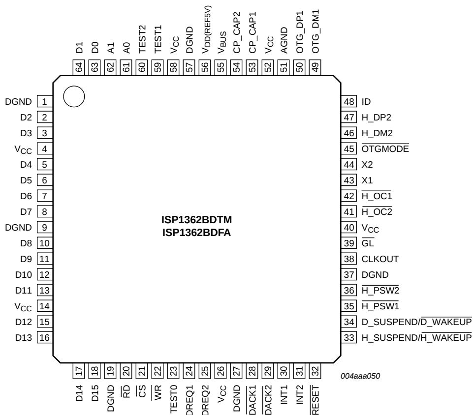
Fig 2. Pin configuration LQFP64
