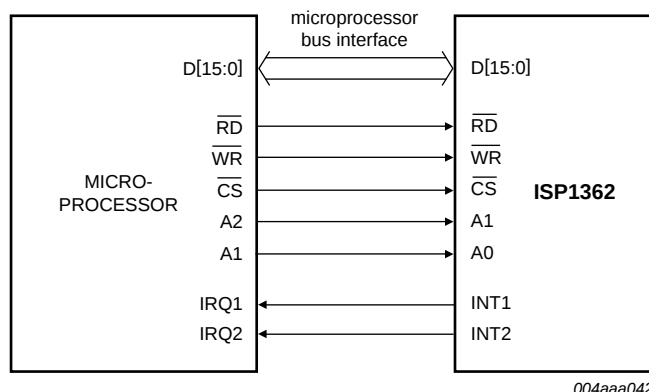
Fig 8. PIO interface between a microprocessor and the ISP1362
