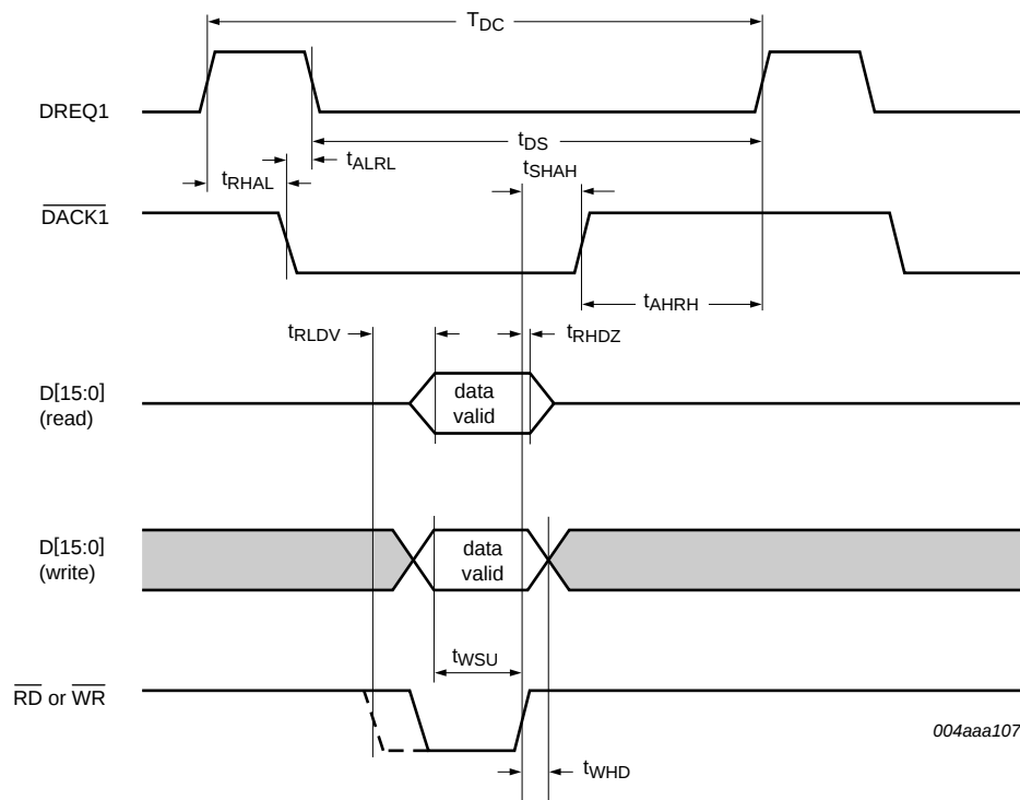
Fig 33. Host controller single-cycle DMA timing
