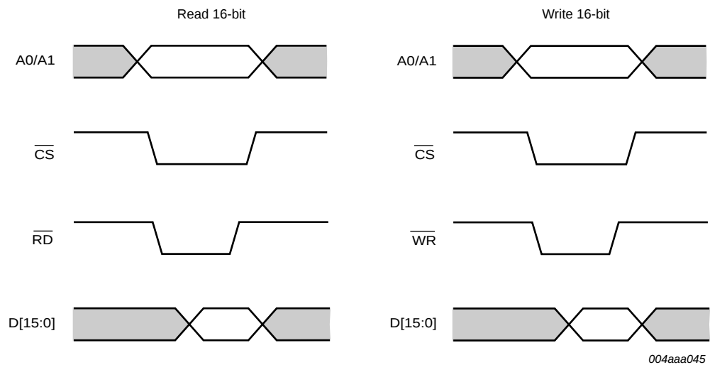
Fig 12. PIO register access
